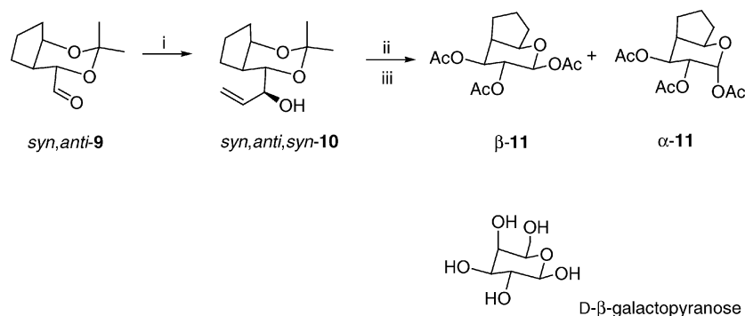
Scheme 6. (i) Vinylmagnesium bromide, THF; (ii) O 3 , MeOH/CH 2 Cl 2 , then PPh 3 ; (iii) THF, H 2 O, 10% HCl.
