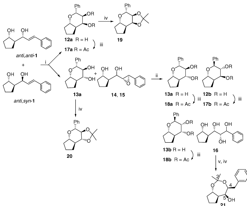
Scheme 7. (i) m CPBA, \text{CH}_2\text{Cl}_2 ; (ii) THF/ \text{H}_2\text{O} , \text{HClO}_4 ; (iii) \text{Ac}_2\text{O} , pyridine; (iv) 2,2-dimethoxypropane, acetone, pyridinium p -toluenesulfonate; (v) \text{H}_2 , Pd/C, EtOH, \text{HClO}_4 .
