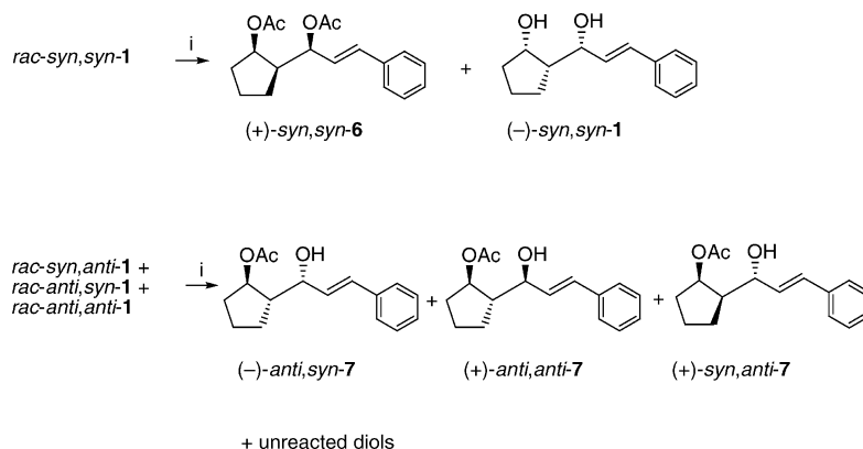
Scheme 4. (i) Baker's yeast, H 2 O/ethanol, glucose; column chromatography.
