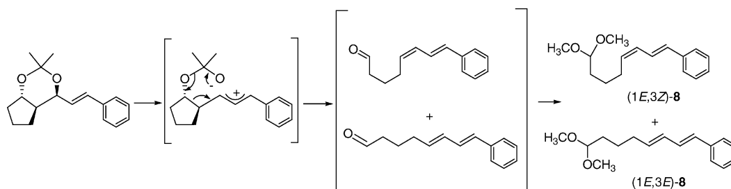
Scheme 5. Acid-catalysed Grob fragmentation.
