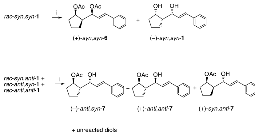
Scheme 3. (i) Lipase PS, tert -butyl methyl ether, vinyl acetate; column chromatography.
