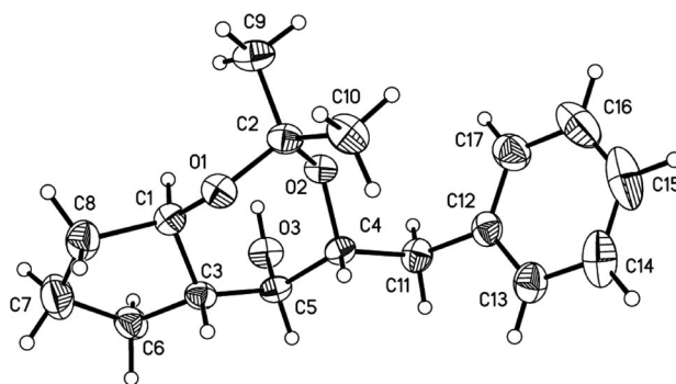
Figure 1. X-ray crystal structure of 21 .
